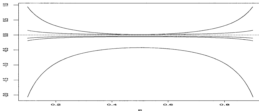
FIG. 2. Comparison of the systematic coverage biases. The y -axis is nS_n(p) . From top to bottom: the systematic coverage biases of the Agresti-Coull, Wilson, Jeffreys, likelihood ratio and Wald intervals, with n = 50 and \alpha = 0.05 .
