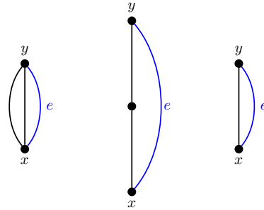
Fig. 1.1 JOIN game CUT game NEUTRAL game
