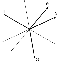
Fig. 1.6 A configuration (V; e) of 4 vectors in general position in \mathbb{R}^2
