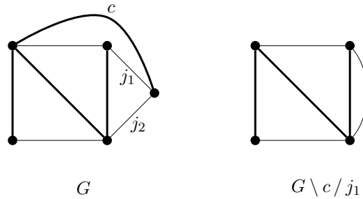
Fig. 1.2 JOIN's response to CUT playing c
