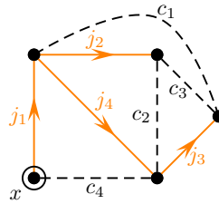
Fig. 1.5 An ARBORESCENCE game on a block played using the strategy of Lemma 2
